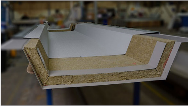
Figure 4: Manufacture of insulated membrane lined valley gutter
