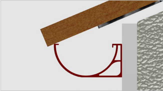
A straight edge can be placed along the pitch of the roof to determine the position of the fascia bracket
