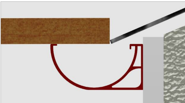
Use a spirit level against the lowest point of the roof tile to determine the position of the fascia bracket
