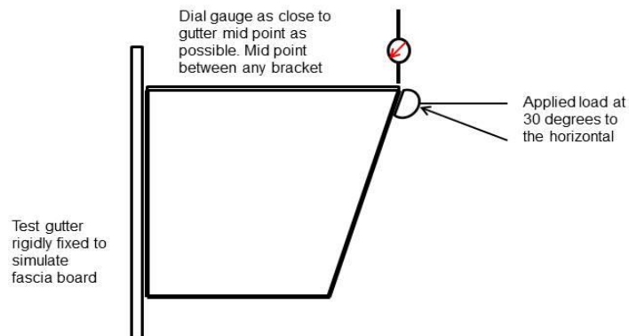
Figure 2 Test equipment for snow load test
