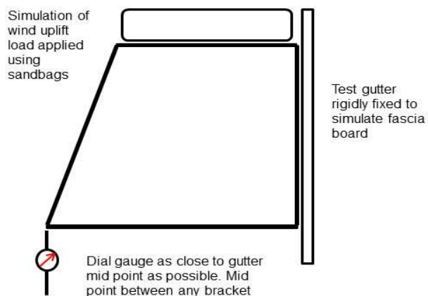
Figure 1 Test equipment for wind uplift test
